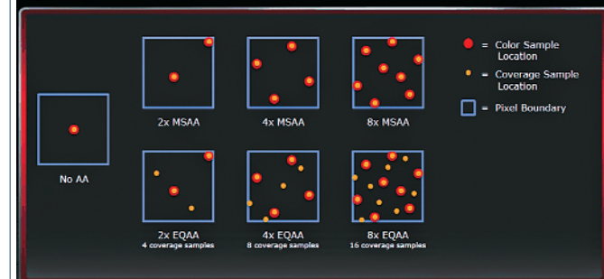
Принцип Enhanced Quality AA и Multi Sampling AA
