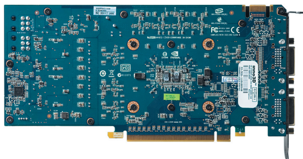
Inno3D GF-GTX460Ti
