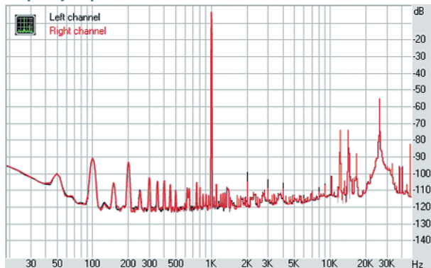
THD + Noise (at -3 dB FS)
